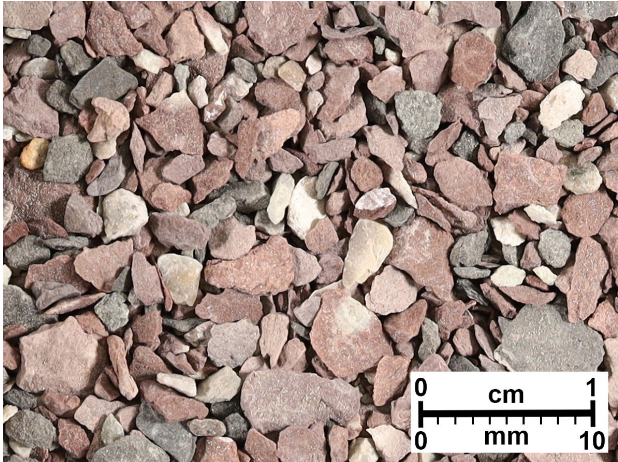
Figure A3. Mudstone/shale, dark red and reddish to purplish orange, soft, clayey to silty, platy; sandstone, tan to gray, very fine to fine grained, sub-angular to sub-rounded, poorly sorted; occasional limestone from limestone nodules; contact with underlying Brushy Basin Member of the Morrison Formation difficult to recognize with cuttings as well as in outcrop when the basal Buckhorn Conglomerate Member is absent because they have near-identical characteristics.
