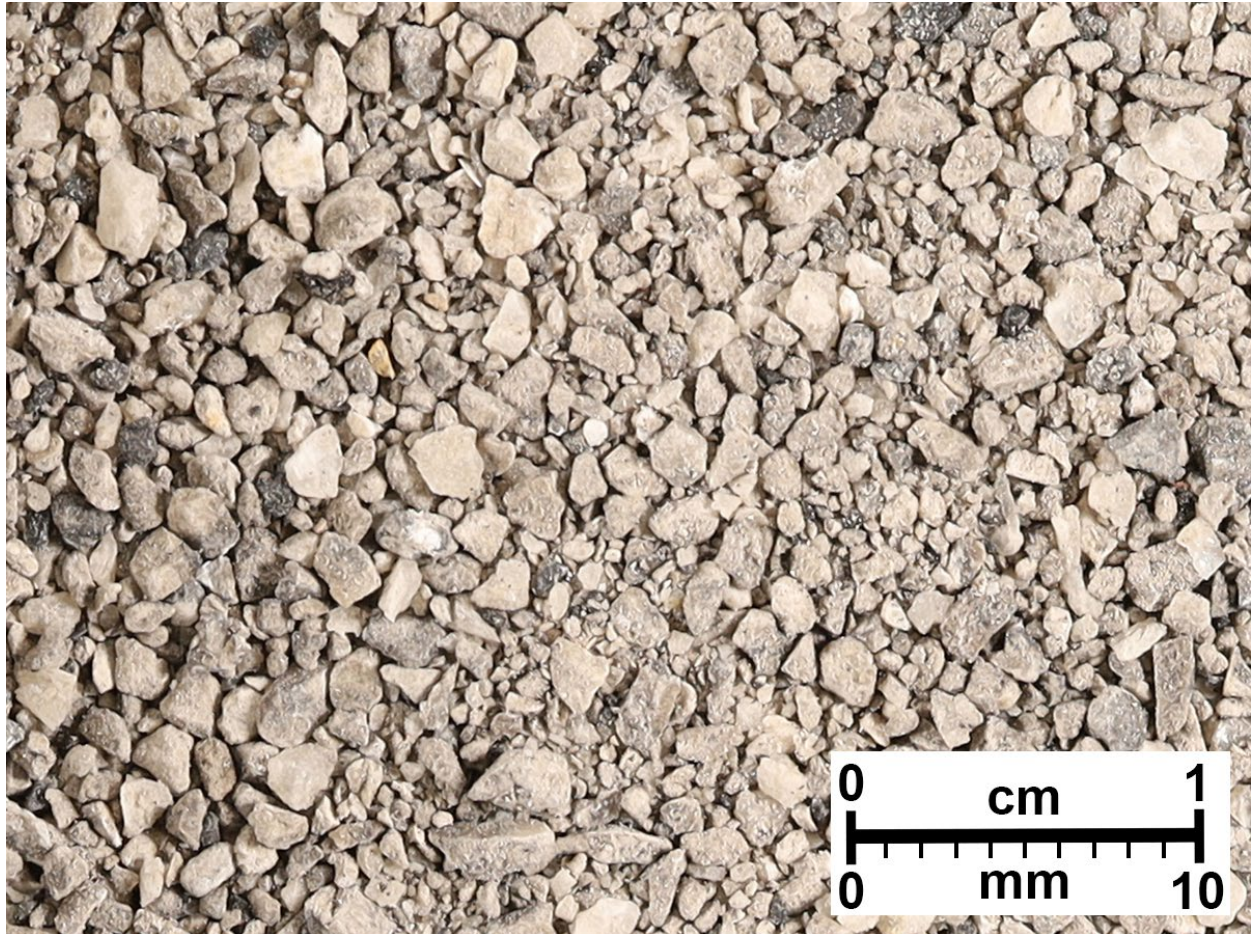
Figure A29. Dolomite, light to dark gray, laminated, argillaceous to shaly in part; shale (10% to 15%), medium to dark gray to black, organic-rich, carbonaceous (sooty); anhydrite (5% to 10%), white, soft to firm, slightly to moderately calcitic.
