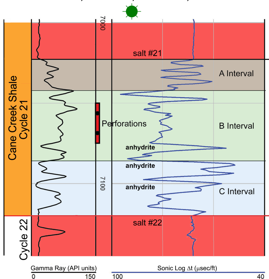
Figure 13. Typical gamma ray-sonic log of the Cane Creek shale, Long Canyon field, Grand County, Utah, showing the divisions of the Cane Creek shale into “A,” “B,” and “C” intervals. Cumulative production from a vertical wellbore in this well (to January 1, 2023) = 1,134,948 barrels of oil, 1.16 billion cubic feet of gas, and 610,423 barrels of water (Utah Division of Oil, Gas and Mining, 2023b). See figure 3 for location of Long Canyon field.
