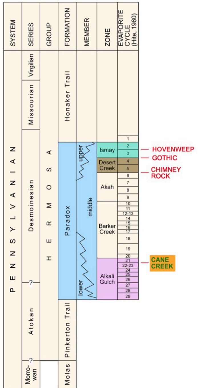
Figure 12. Stratigraphic column for the Paradox Basin; cycles and informal zones with significant production are highlighted with colors. Note the position of the Cane Creek shale, which occurs below the U.S. Geological Survey’s Hovenweep, Gothic, and Chimney Rock Shale Oil and Gas Assessment Units (2012) in the Paradox Basin (also see Chidsey, 2016). Modified from Hite (1960), Hite and Cater (1972), and Reid and Berghorn (1981).
