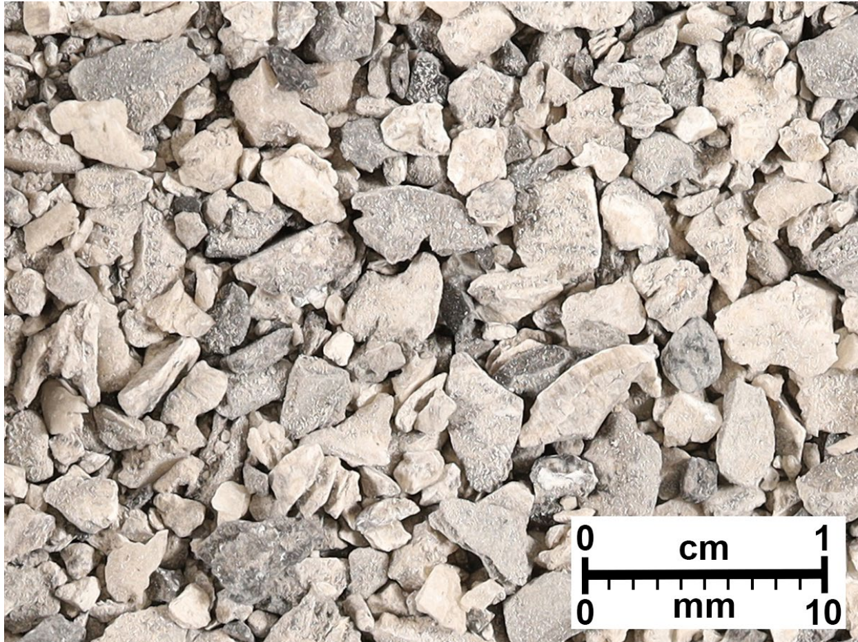
Figure A36. Halite, white to opaque to light brown, coarse, crystalline, brittle to hard; dolomite, light to medium gray, laminated to massive, calcareous to anhydritic, silty to organic-rich, mudstone; shale, black, dense, organic-rich.
