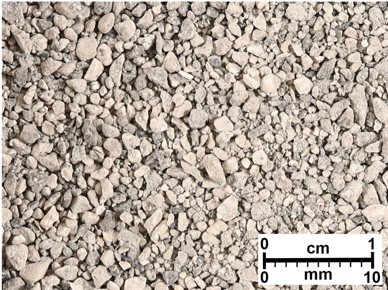
Figure A28. Dolomite, light to dark gray, laminated, argillaceous to shaly; shale (10% to 15%), medium to dark gray, organic-rich, carbonaceous (sooty); anhydrite (5% to 10%), white, soft to firm, slightly to moderately calcitic.
