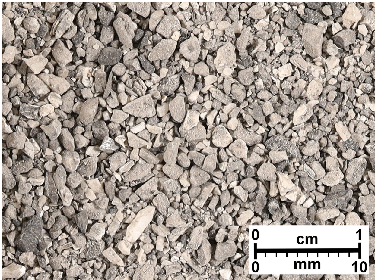
Figure A32. Shale, black to dark gray, soft to firm, organic-rich, carbonaceous (sooty), bitumen, calcareous; dolomite, light to medium gray, chalky to micro sucrosic; anhydrite, light gray to white, soft, chalky; halite.
