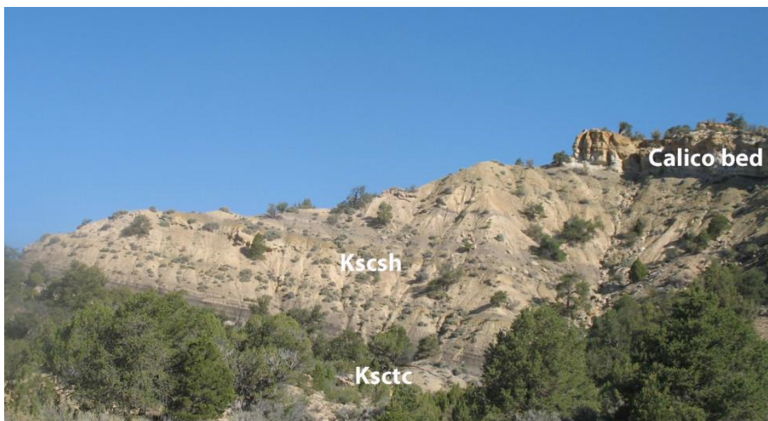
Figure 28. The Smoky Hollow Member (Kscsh) overlies the nearshore deposits of the Tibbet Canyon Member (Ksctc); note the carbonaceous horizons low in the Smoky Hollow Member. The Smoky Hollow is capped by the sandstones and conglomerates of the Calico bed.
