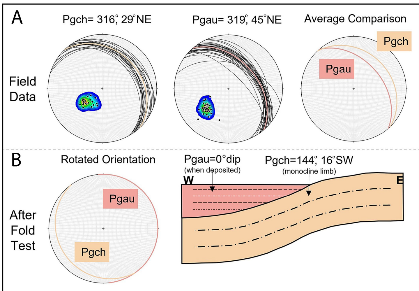
Figure 7. (A) Stereonet plots showing the average bedding attitude from measurements taken from the Crazy Hollow Formation and the formation of Aurora in the vicinity of the mapped area shown in Figures 4 and 5. Field data from the Crazy Hollow show an average orientation of 316°, dip 29° NE. (N. 44° W., dip 29° NE.), whereas field data from the Aurora show an average orientation of 319°, dip 45° NE. (N. 41° W., dip 45° NE.). (B) Raw field data of Aurora strata were rotated back to horizontal (a fold test) to determine the orientation of the Crazy Hollow Formation at the time the Aurora was being deposited. When the Aurora was horizontal (0° dip), the Crazy Hollow was oriented 144°, dip 16° SW. (S. 36° E., dip 16° SW.). An idealized cross section (without antithetic normal faults) shows the discordant relationship between Crazy Hollow and Aurora strata.
