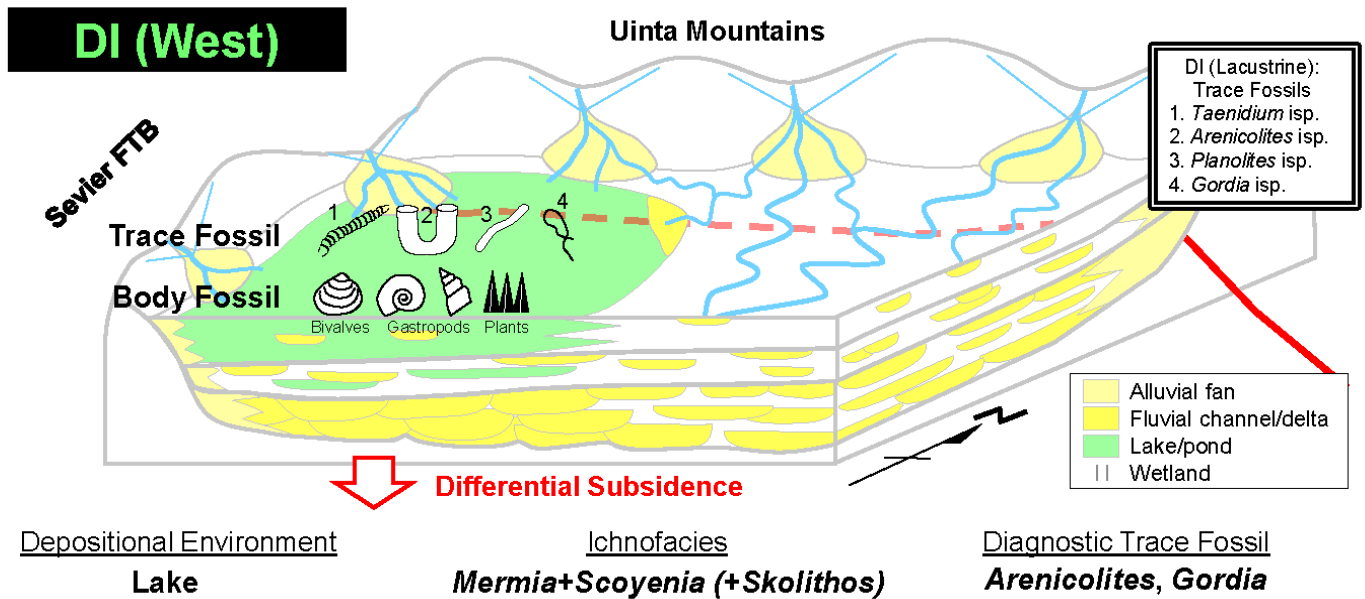
Figure 14. Paleoenvironmental reconstruction and trace fossil assemblage of Dl. An extensive lake environment developed during the deposition of Dl. The trace fossil association in this unit indicates a mixture of the Mermia , Scoyenia , and Skolithos ichnofacies, demonstrating the recurrence of lacustrine communities.
