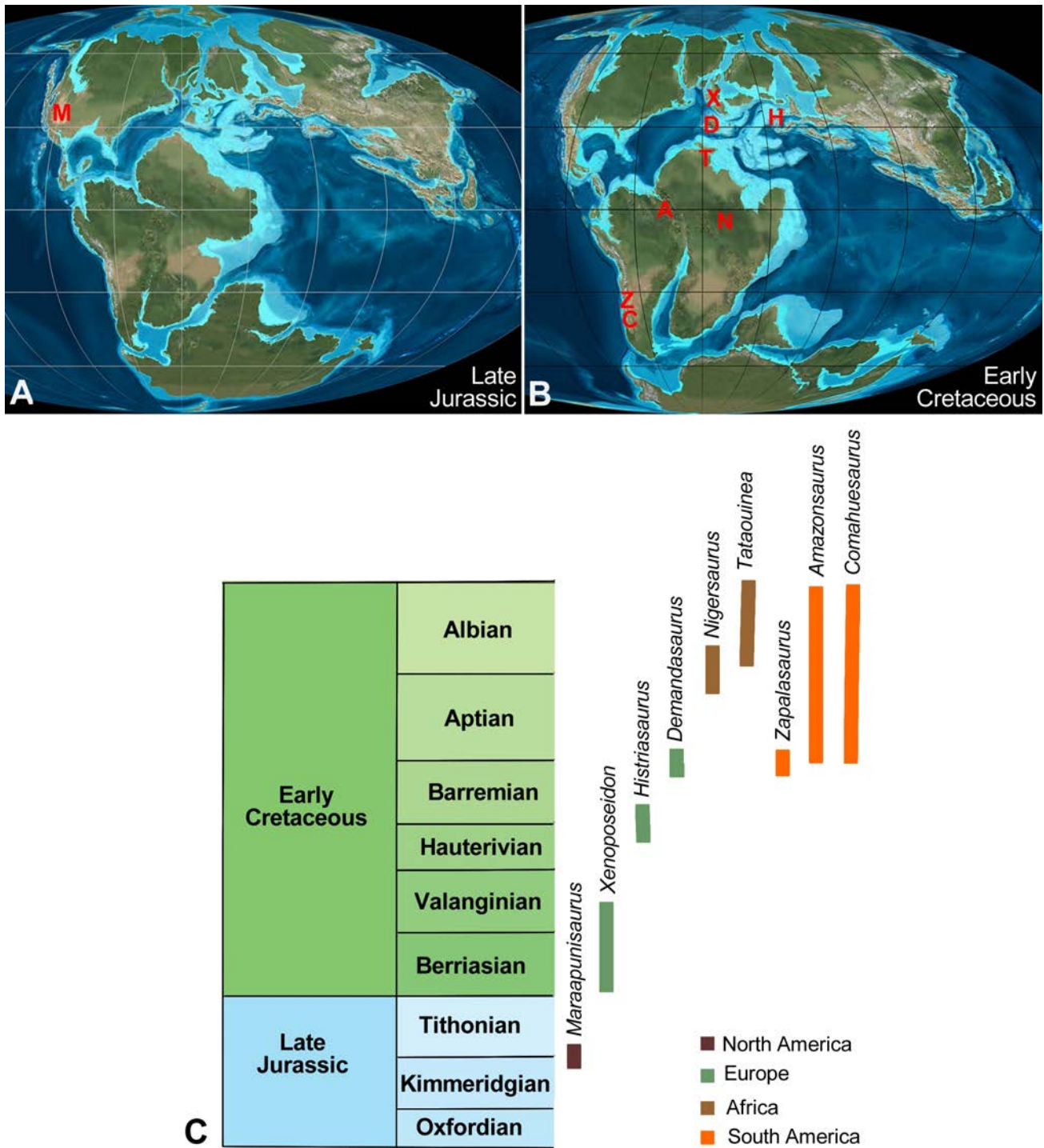
Figure 8. Paleogeographic maps showing the distribution of rebbachisaurids during the Late Jurassic (A) and Early Cretaceous (B). Abbreviations: M– Maraapunisaurus (Kimmeridgian-Tithonian), A– Amazonsaurus (Aptian-Albian), C– Comahuesaurus (Aptian-Albian), D– Demandasaurus (Upper Barremian-Lower Aptian), H– Histriasaurus (Upper Hauterivian-Lower Barremian), N– Nigersaurus (Aptian-Albian), T– Tataouinea (Albian), X– Xenoposeidon (Berriasian-Valanginian), and Z– Zapalasaurus (Barremian-lower Aptian). (C) Temporal and paleogeographic distribution of Late Jurassic and Early Cretaceous rebbachisaurids. Paleogeographic maps from the commercial version of Ron Blakey’s “Paleogeography of Western North America” that is licensed to the Prehistoric Museum.
