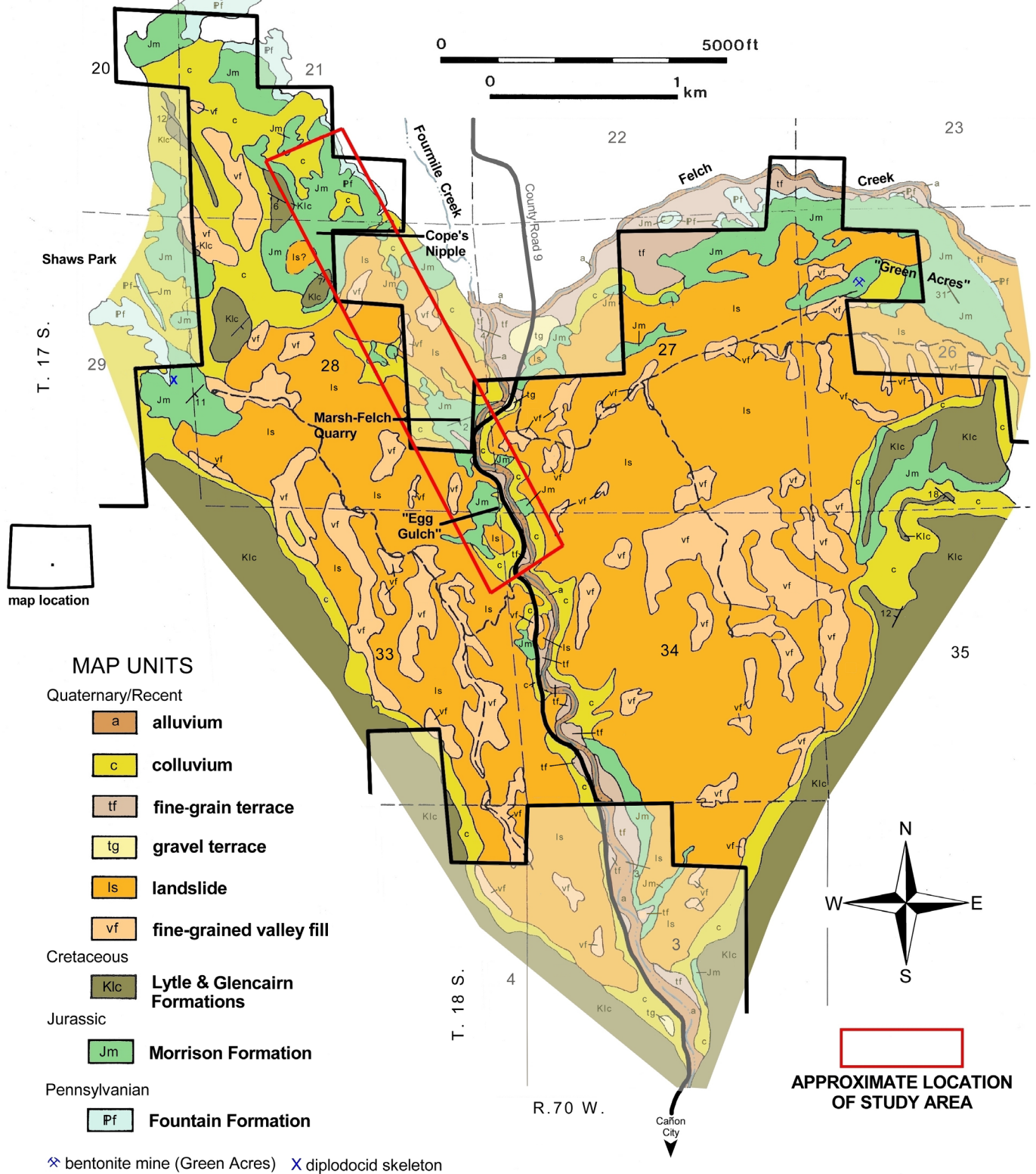
Figure 1. Simplified geological map of the Garden Park National Natural Landmark, which is about 9 km north of Cañon City, Colorado. Map courtesy of E. Evanoff (University of Northern Colorado).
