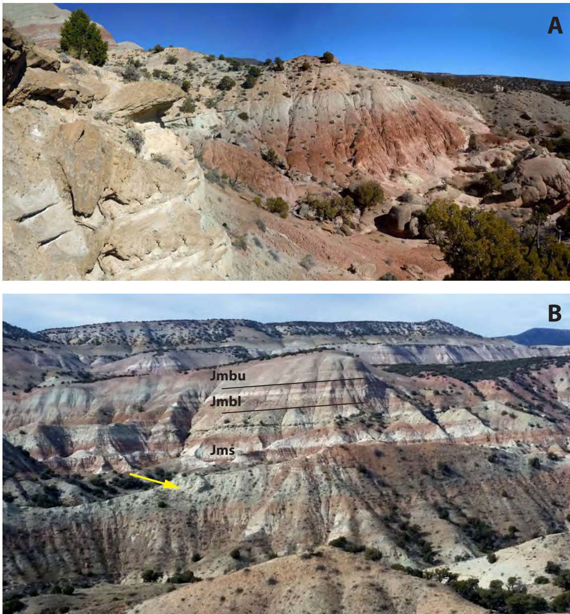
Figure 7. Photographs of the Salt Wash and Brushy Basin Members of the Morrison Formation. (A) Salt Wash Member near the measured section at Miners Draw showing varicolored siltstone beds and the brownish-gray channel sandstone beds; view to the northeast. (B) View of the Salt Wash and Brushy Basin Members from near the top of the measured section at Rainbow Draw; view to the west. The yellow arrow points to the fossil log-bearing interval, which is overlain by the reddish-colored marker bed. The Brushy Basin is divided into a lower banded unit and an upper gray unit. The Cretaceous Cedar Mountain through the Frontier Formations are exposed on the distant ridge.
