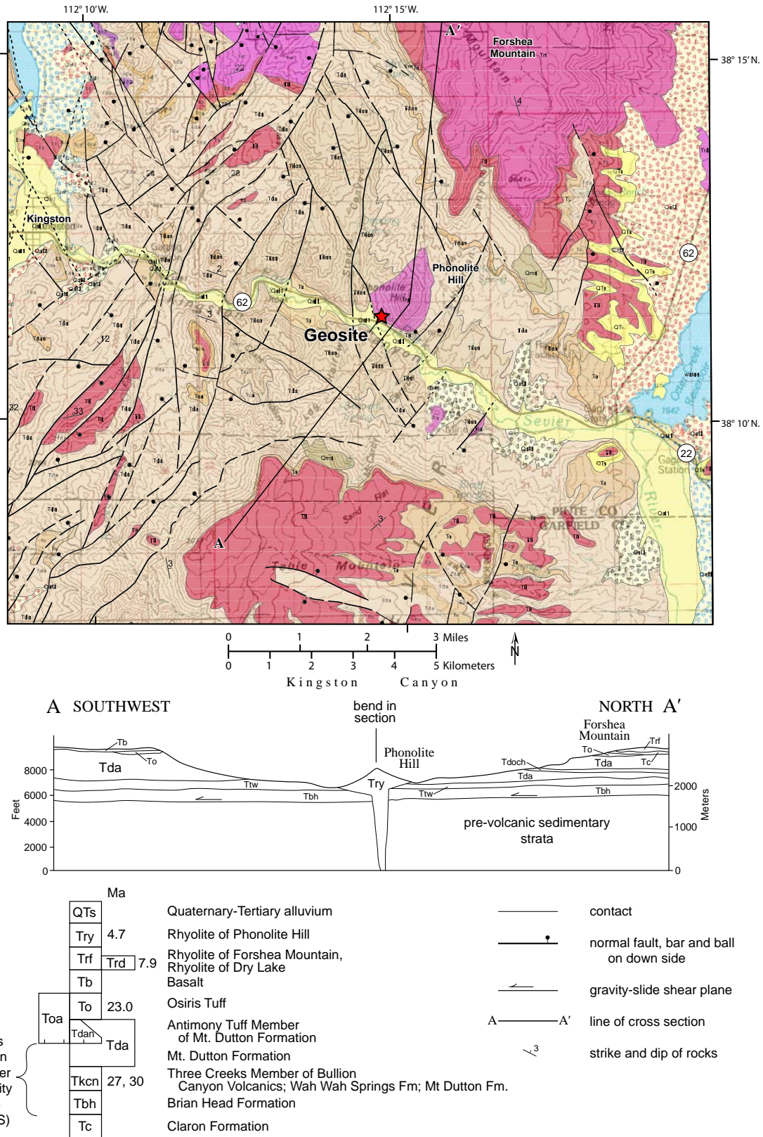
Figure 2. Geologic map and cross section of the Kingston Canyon area, Piute and Garfield Counties, Utah, showing Phonolite Hill. Cross section shows Phonolite Hill erupted at the base of Kingston Canyon. Geologic map modified from Rowley and others (2005).
