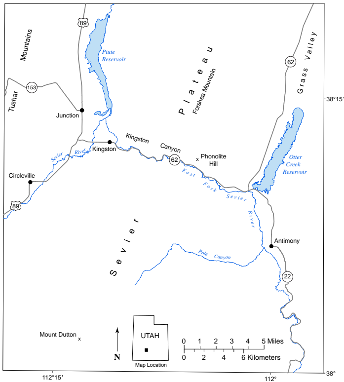
Figure 1. Location map of the Kingston Canyon area, Piute and Garfield Counties, Utah, with the Phonolite Hill geosite identified.
