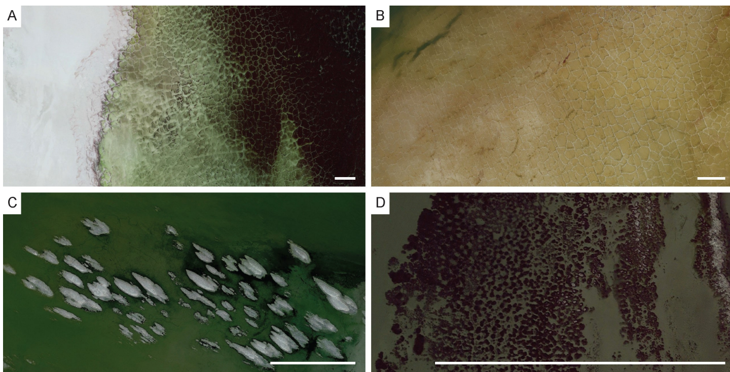
Figure 7. Examples of field-verified microbialite reef areas identified from remote imagery in the south arm of Great Salt Lake. (A) Dark green submerged microbialites and bright bleached megapolygons indicate the presence of microbialites in a nearshore area in the south arm of the lake (41.073°, -112.573°). (B) Submerged desiccated microbialite-edged polygons in the north arm of the lake (41.249°, -112.533°). (C) Bright exposed and desiccated microbialites stand out against green lake water at a site near the Antelope Island marina (41.064°, -112.237°). (D) Partially submerged microbialites between Buffalo Point and White Rock Bay (41.033°, -112.275°). Scale bar in all images is 100 m. Image locations are shown as markers on the map in Fig. 8. Images from Google Earth Pro.
