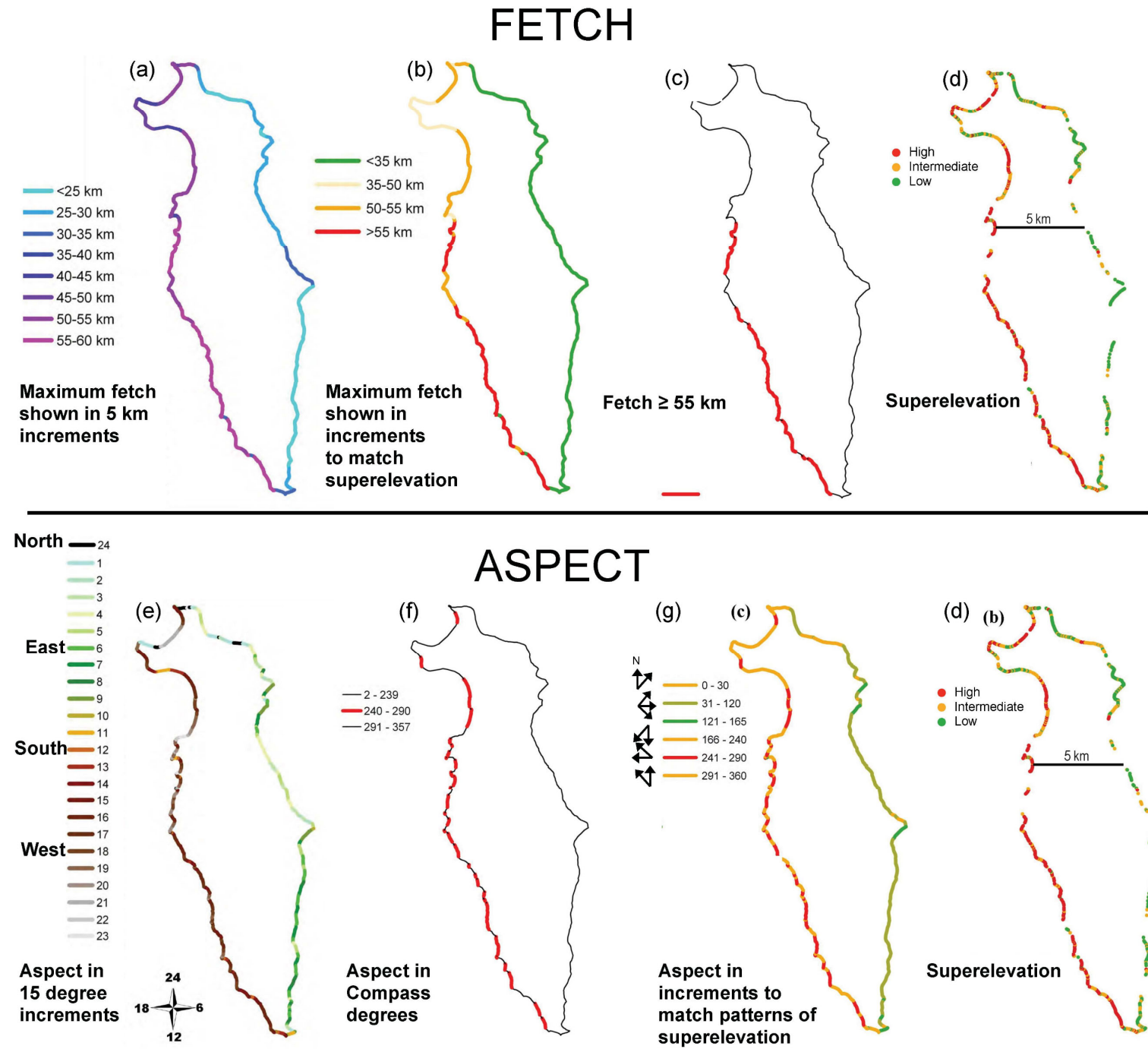
Figure 6. Associations of shoreline superlevation with fetch and aspect. The two sets of maps show associations of maximum fetch, aspect in 15-degree increments, and shoreline superlevation. Visual inspection indicated correlations among shoreline superlevation, fetch, and aspect. Adapted from Atwood (2006).
