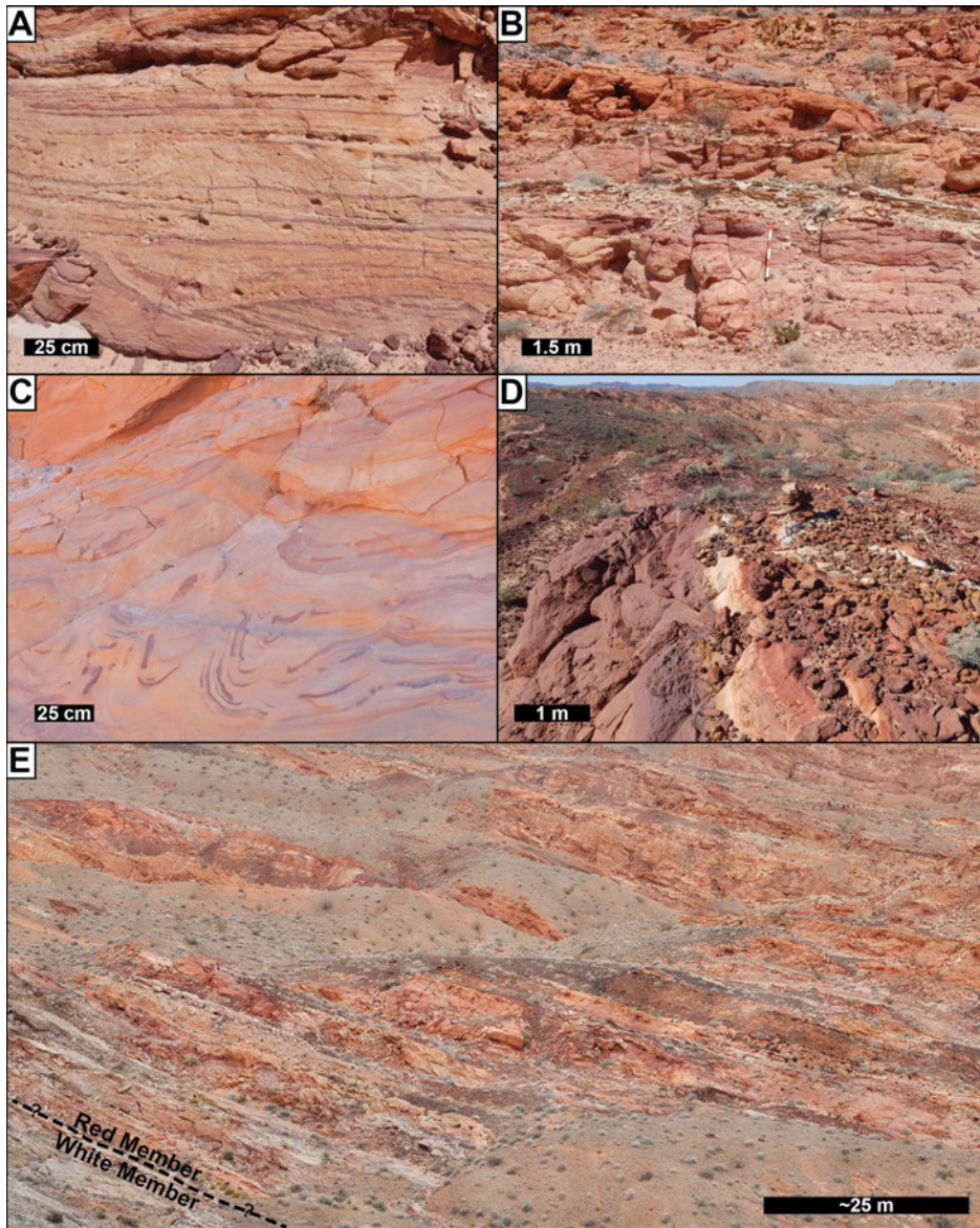
Figure 4. Coloration facies of the lower red sandstone member (Kbr). (A) Red and purple coloration, with increased concentration at cross-stratification surfaces. (B) Range of red and purple to white/tan coloration characteristic of the member (Jacob's staff near image center 1.5 m tall with each red/white bar = 25 cm). (C) Purple coloration patterns found along soft-sediment deformation surfaces. (D) Intensely concentrated red and purple coloration. (E) Perspective view of the lower red sandstone member in the study area (about 75 m of section), showing the range of colors and general bedding-parallel concentration of colors.
