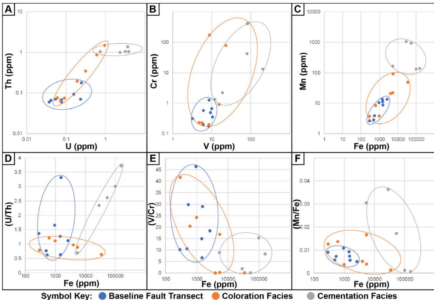
Figure 11. Cross-plots of elemental concentrations for key redox-sensitive elements as measured using ICP-MS. The A through C simple cross-plots show that the Baseline Fault Transects samples (BFT) and the cementation facies overlap with coloration but do not overlap each other. In D through F, elemental ratios are plotted against iron concentration to normalize for concentration effects; note that the distinct plotting areas of the BFT and cementation facies samples remain.
