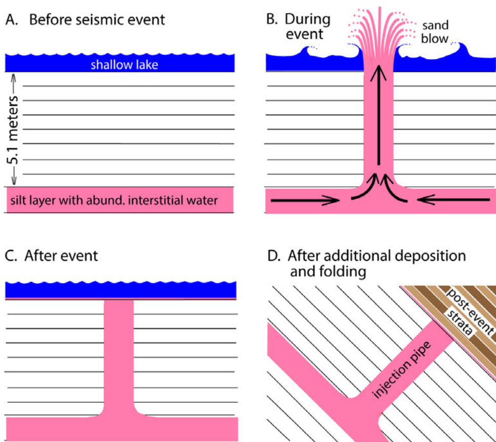
Figure 6. Schematic 4-stage model for the development of the Lovell Wash clastic pipe.
